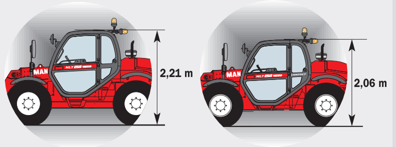
LOW PROFILE CAB "Compact" version (Atmo or Turbo)
